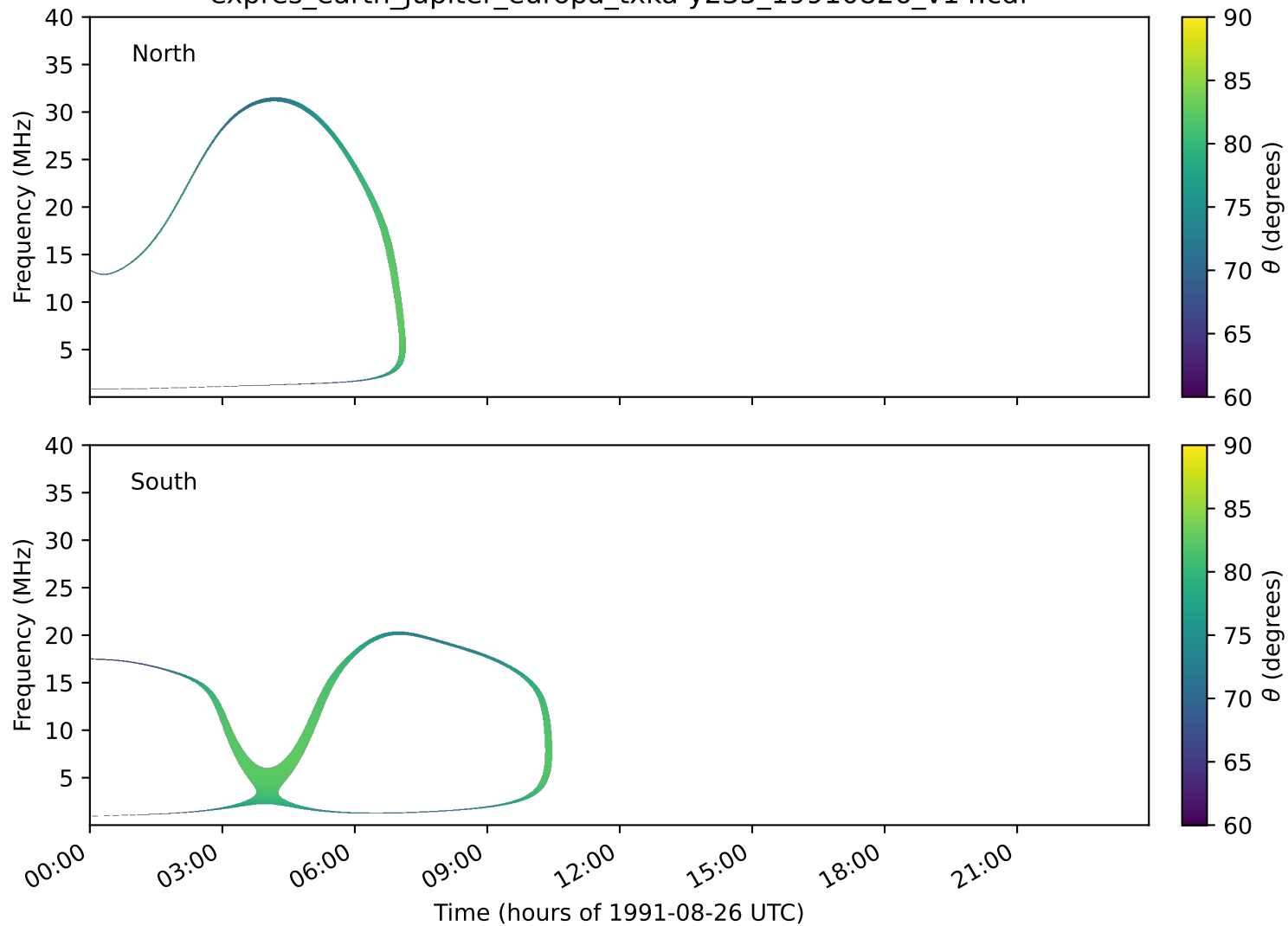
expres_earth_jupiter_europa_txka-y235_19910826_v14.cdf
