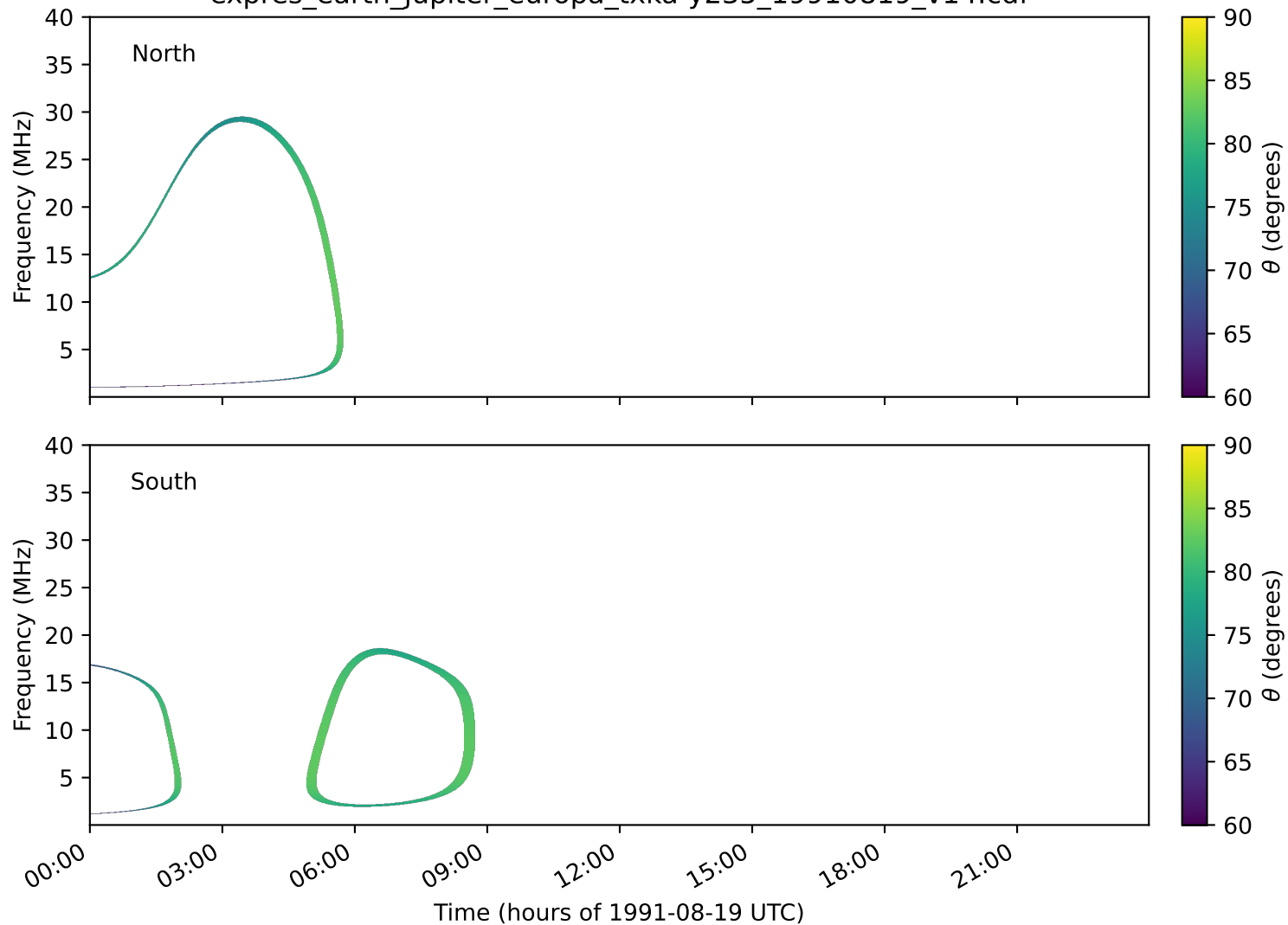
expres_earth_jupiter_europa_txka-y235_19910819_v14.cdf
