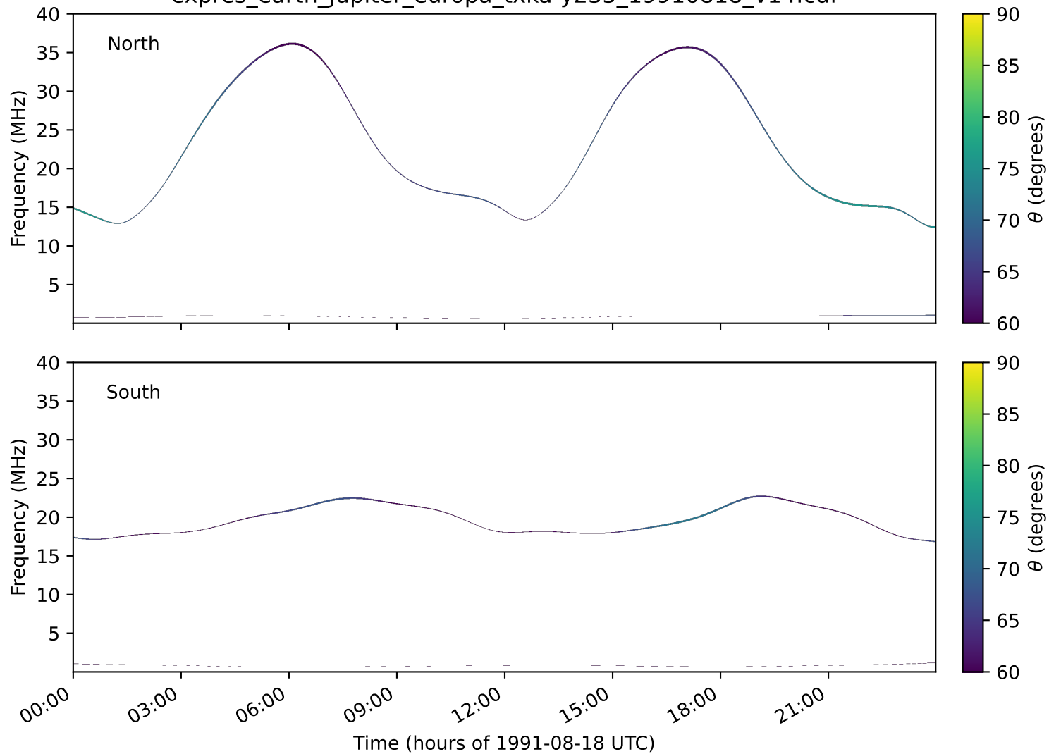
expres_earth_jupiter_europa_txka-y235_19910818_v14.cdf
