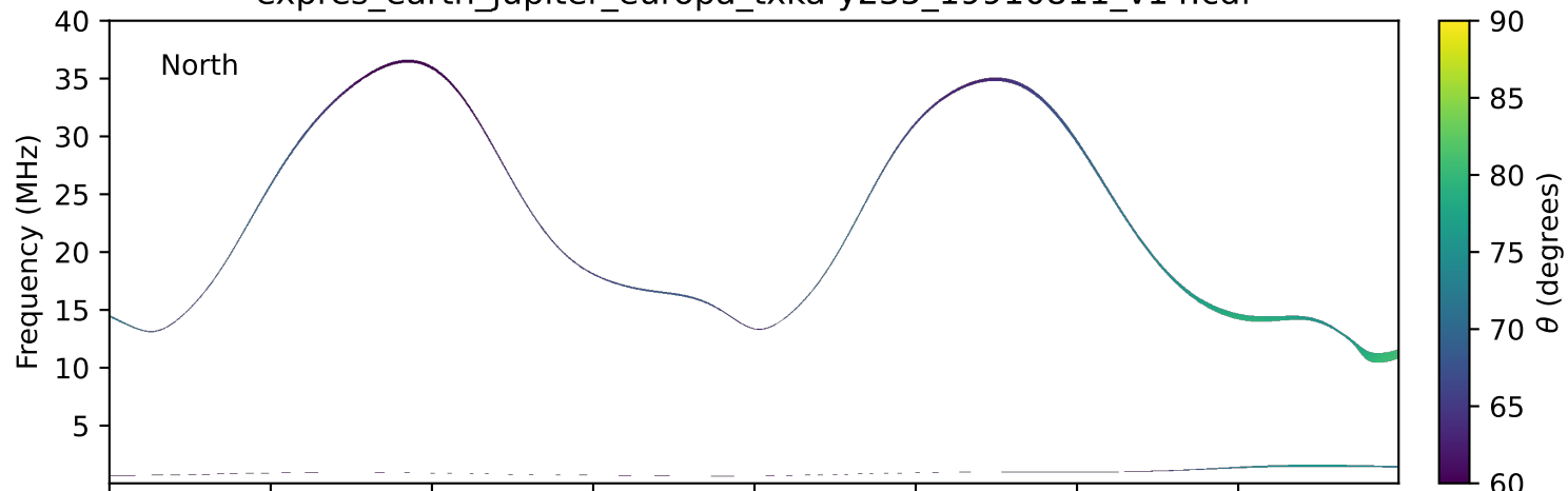
expres_earth_jupiter_europa_txka-y235_19910811_v14.cdf
