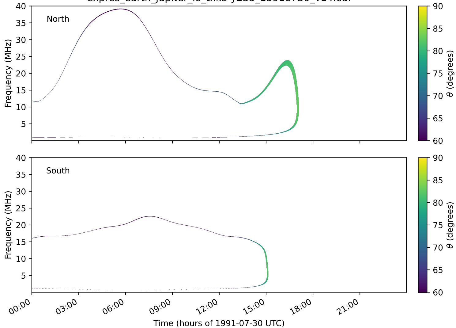
expres_earth_jupiter_io_txka-y235_19910730_v14.cdf
