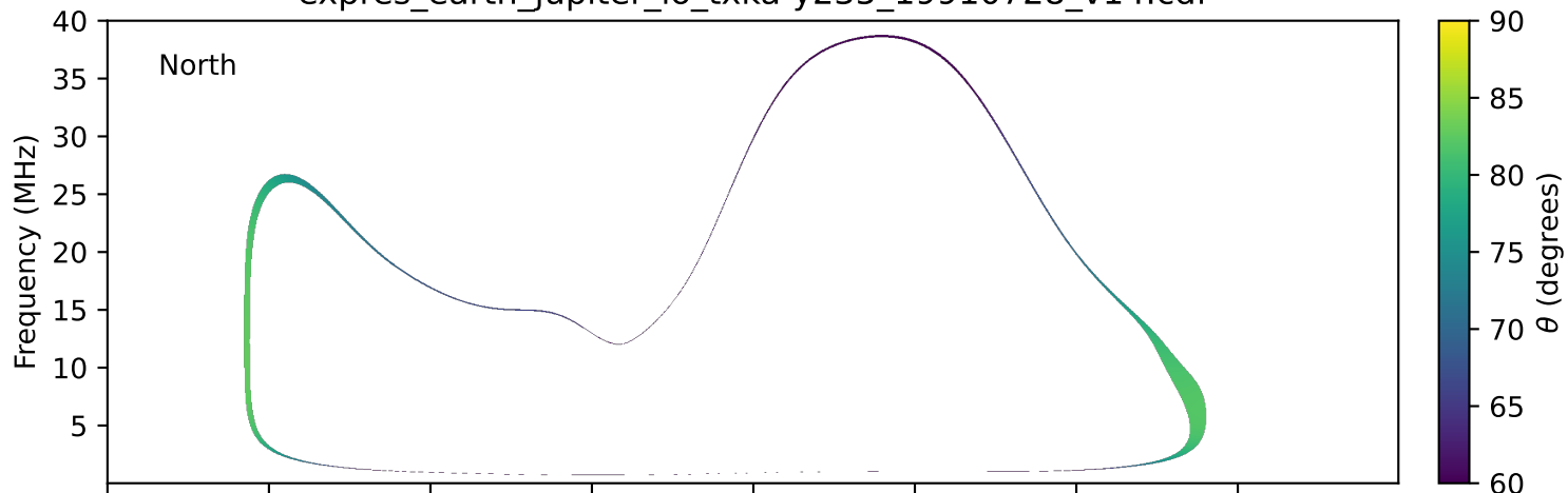
expres_earth_jupiter_io_txka-y235_19910728_v14.cdf
