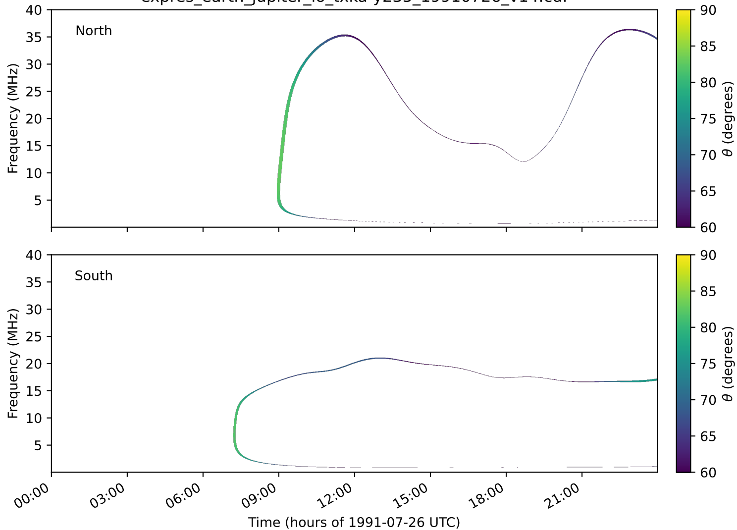
expres_earth_jupiter_io_txka-y235_19910726_v14.cdf
