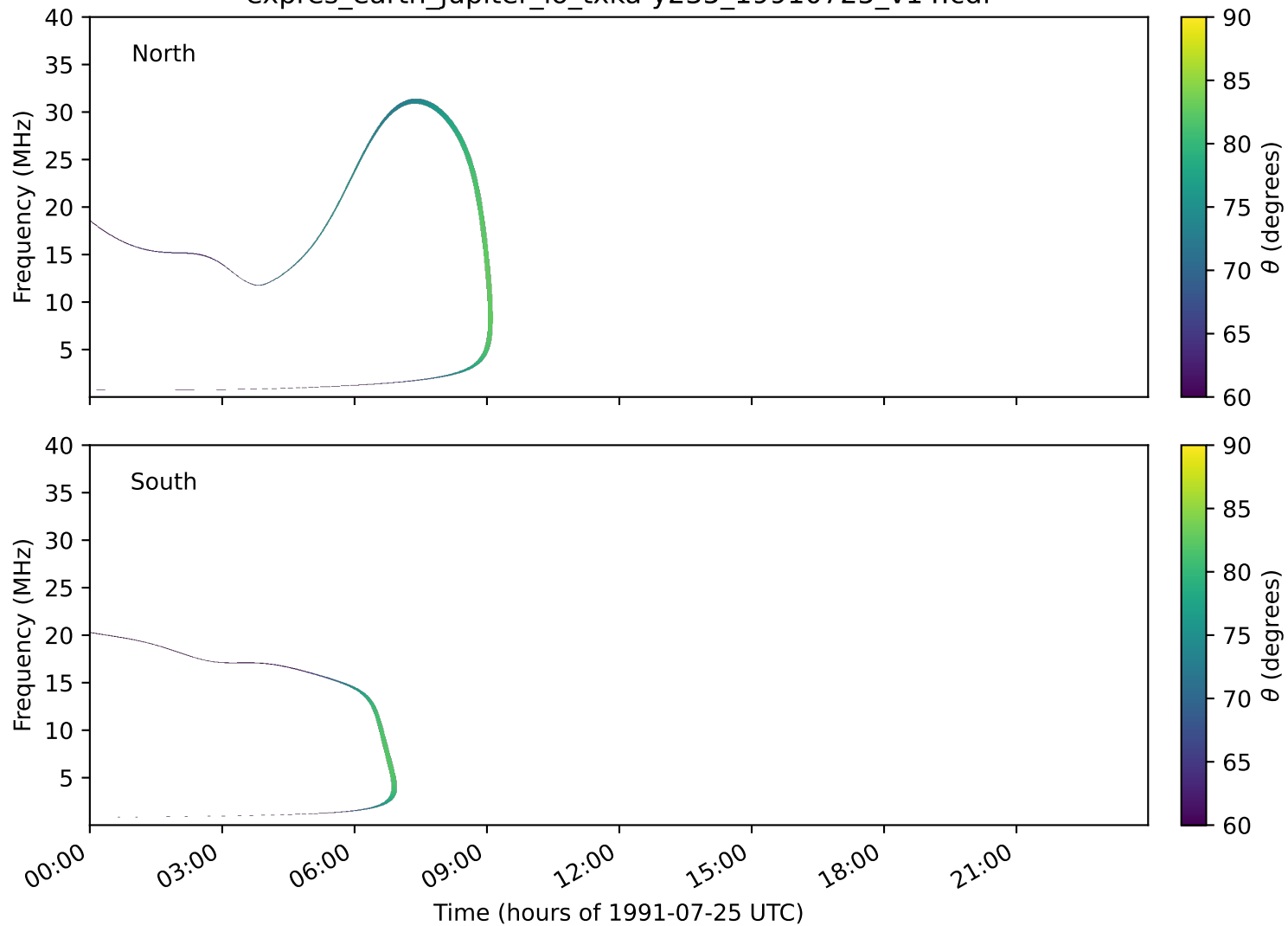
expres_earth_jupiter_io_txka-y235_19910725_v14.cdf
