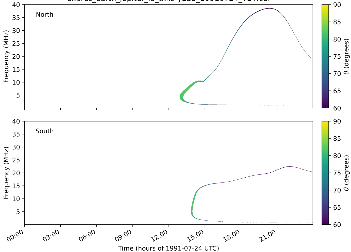
expres_earth_jupiter_io_txka-y235_19910724_v14.cdf
