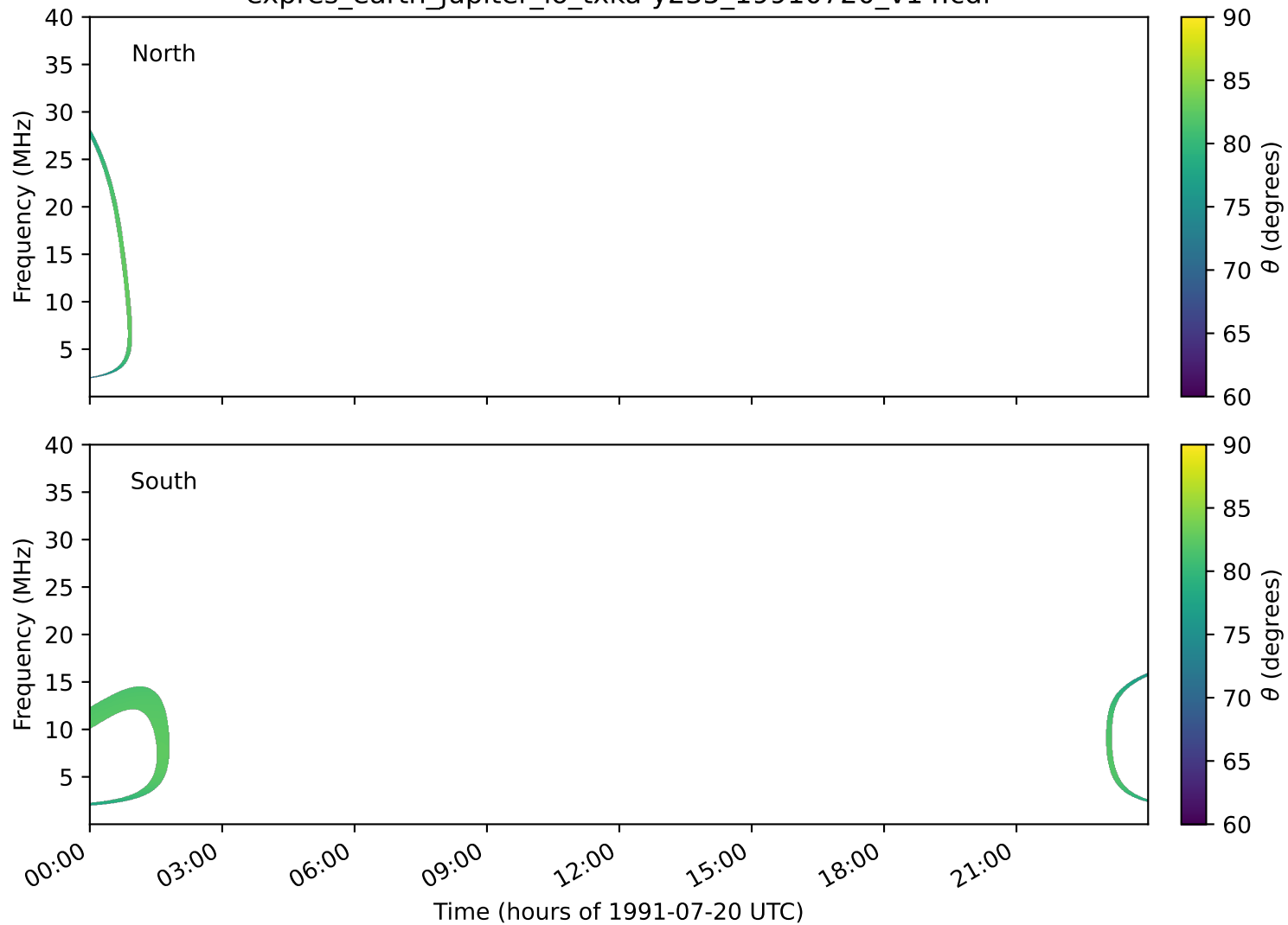
expres_earth_jupiter_io_txka-y235_19910720_v14.cdf
