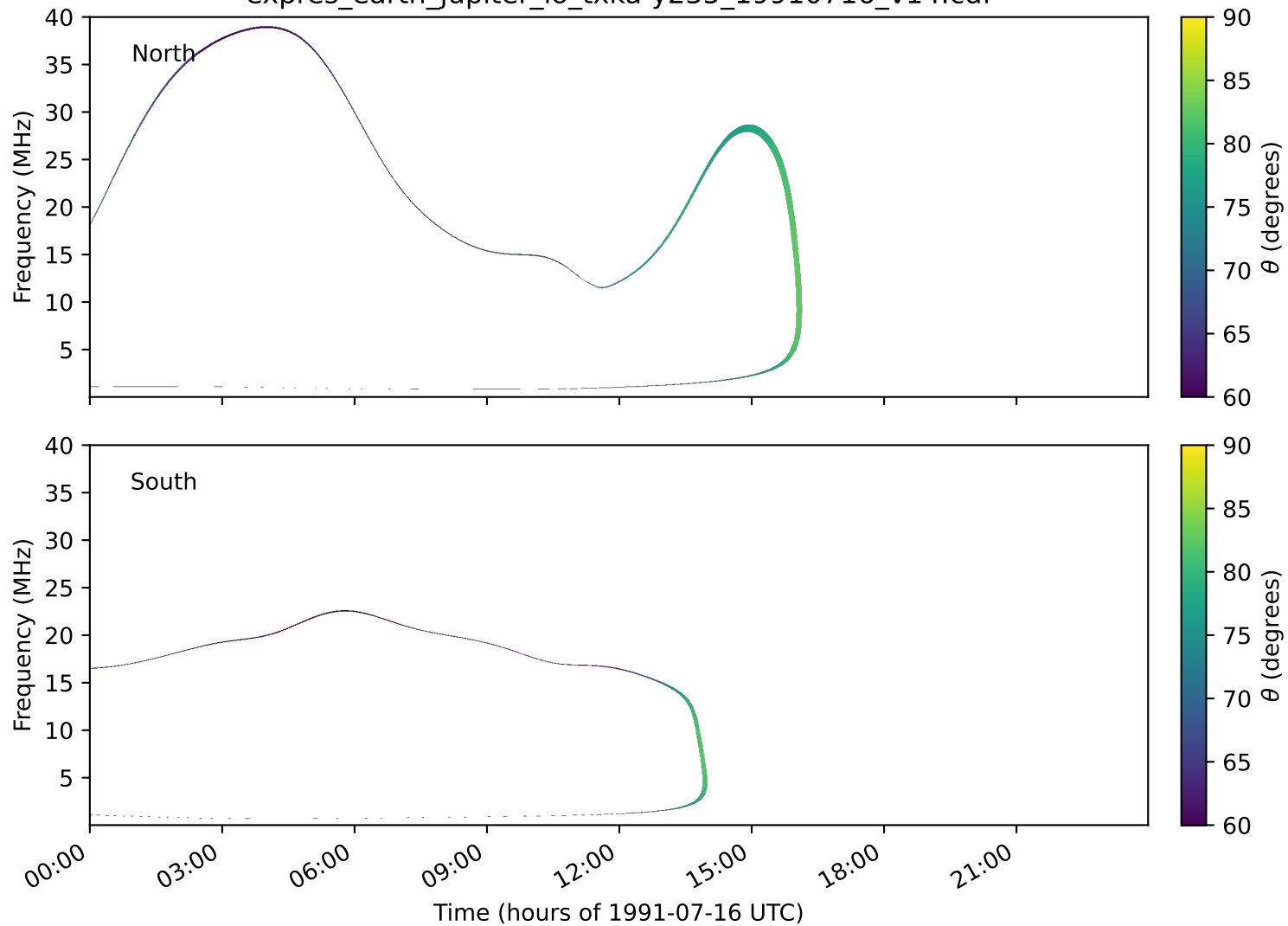
expres_earth_jupiter_io_txka-y235_19910716_v14.cdf
