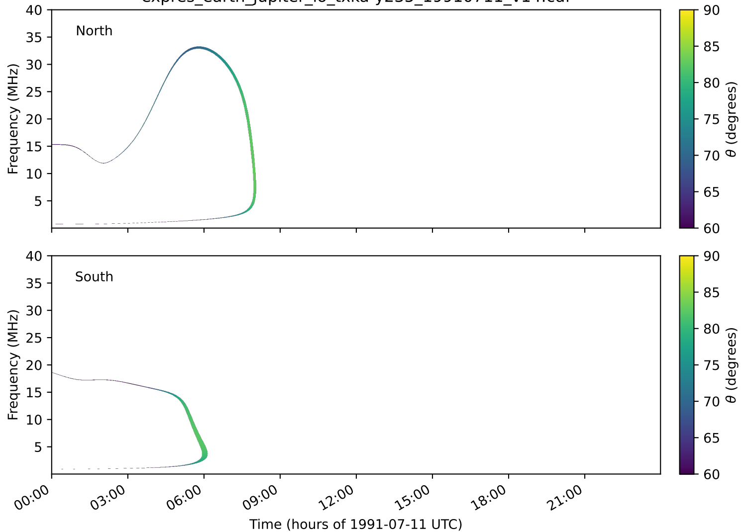
expres_earth_jupiter_io_txka-y235_19910711_v14.cdf
