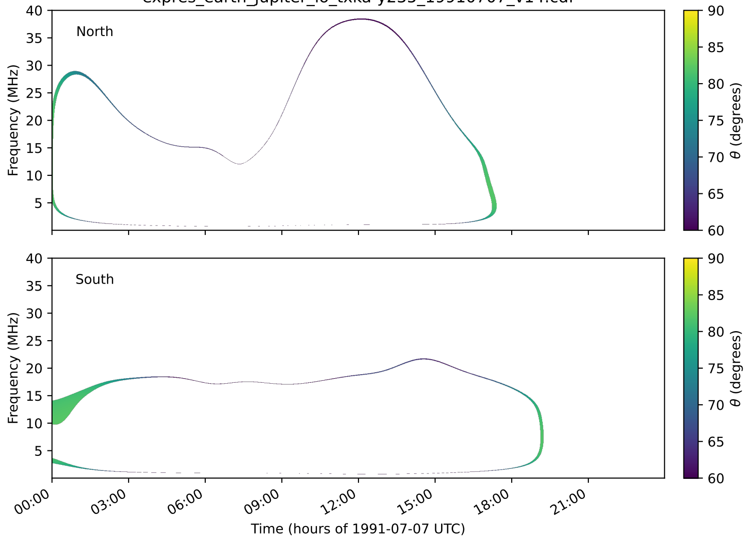
expres_earth_jupiter_io_txka-y235_19910707_v14.cdf
