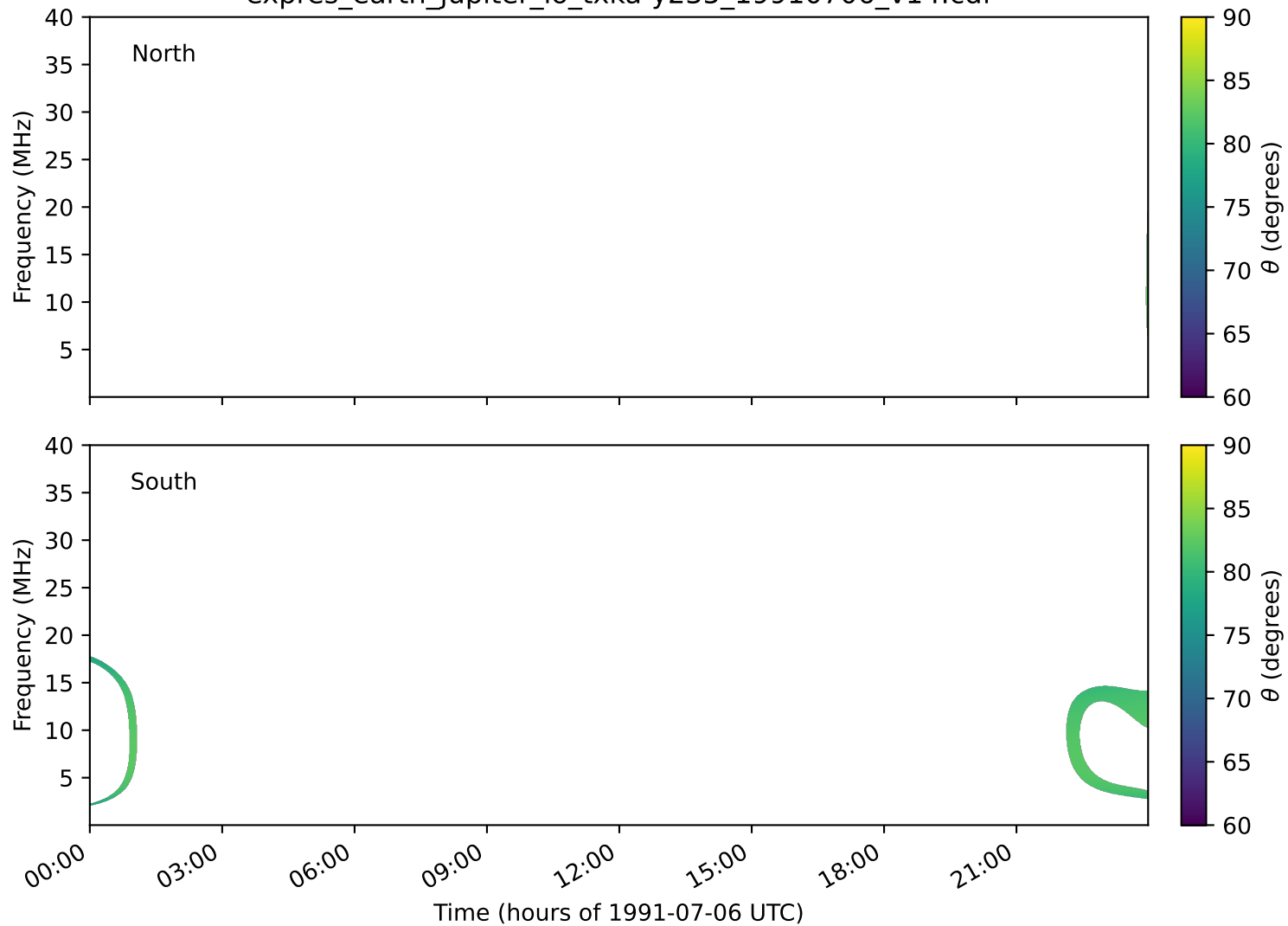
expres_earth_jupiter_io_txka-y235_19910706_v14.cdf
