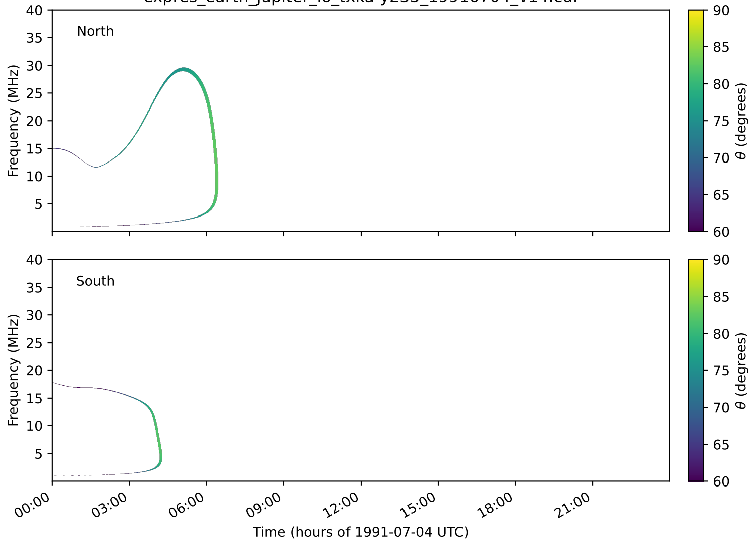
expres_earth_jupiter_io_txka-y235_19910704_v14.cdf
