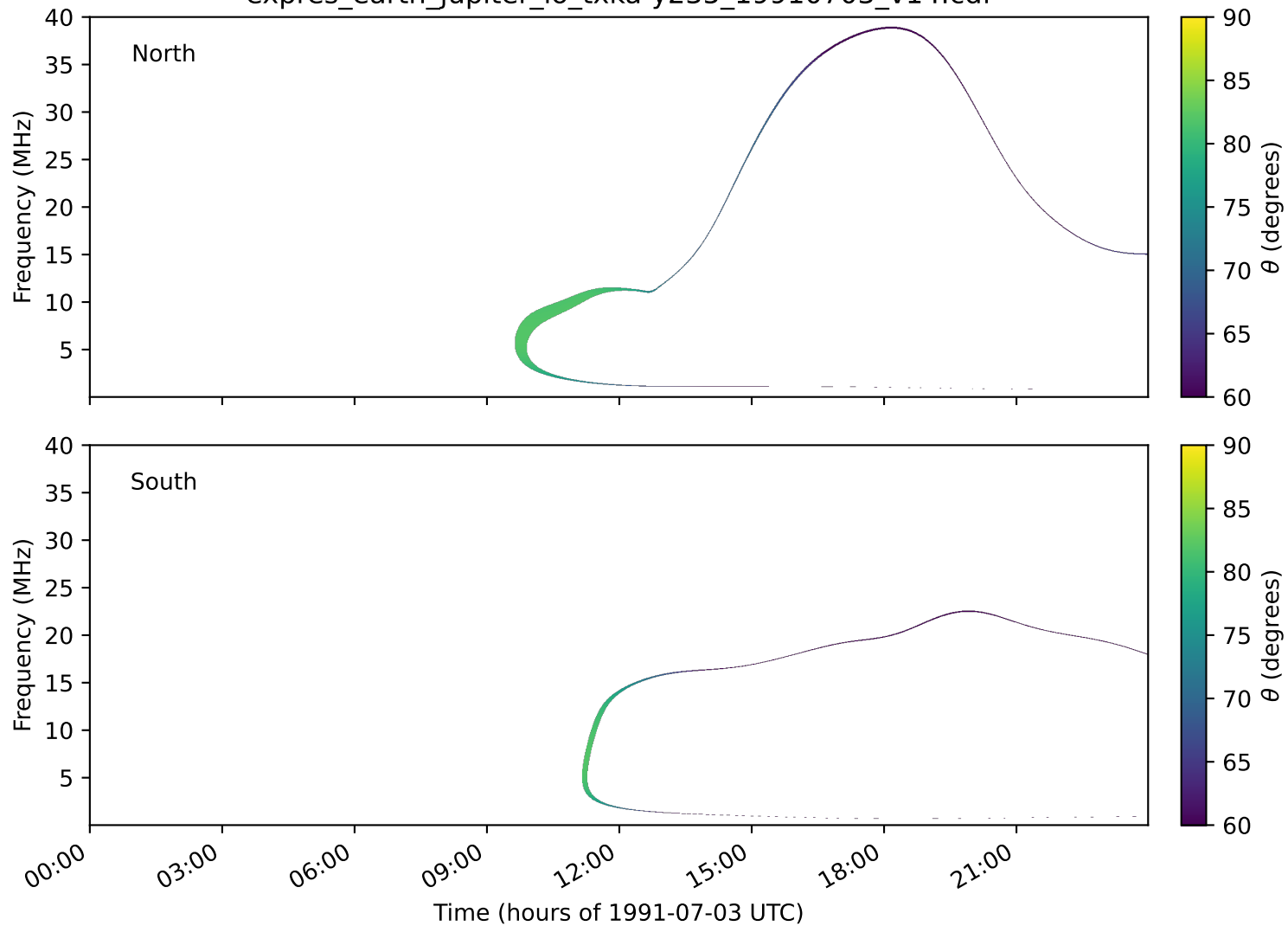
expres_earth_jupiter_io_txka-y235_19910703_v14.cdf
