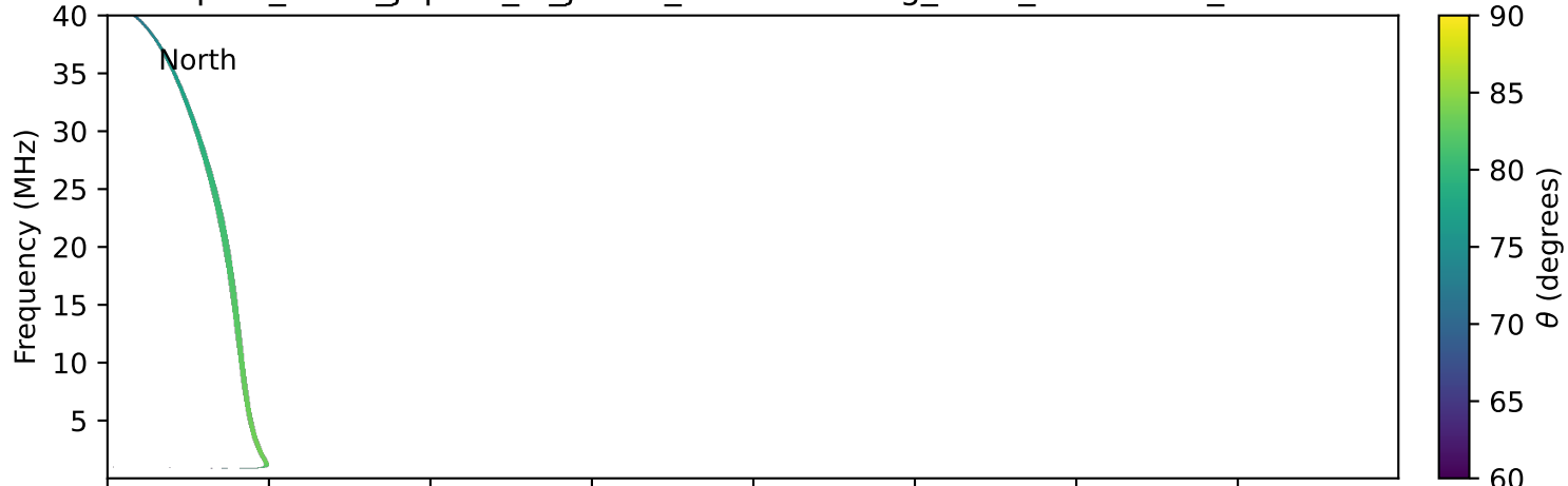
expres_earth_jupiter_io_jrm33_lossc-wid1deg_3kev_19910727_v11.cdf
