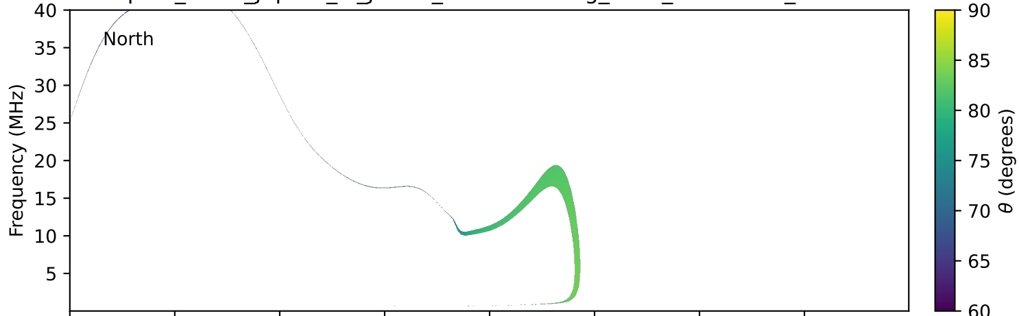
expres_earth_jupiter_io_jrm33_lossc-wid1deg_3kev_19910709_v11.cdf
