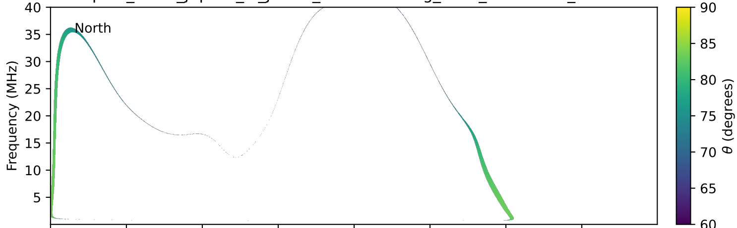
expres_earth_jupiter_io_jrm33_lossc-wid1deg_3kev_19910707_v11.cdf
