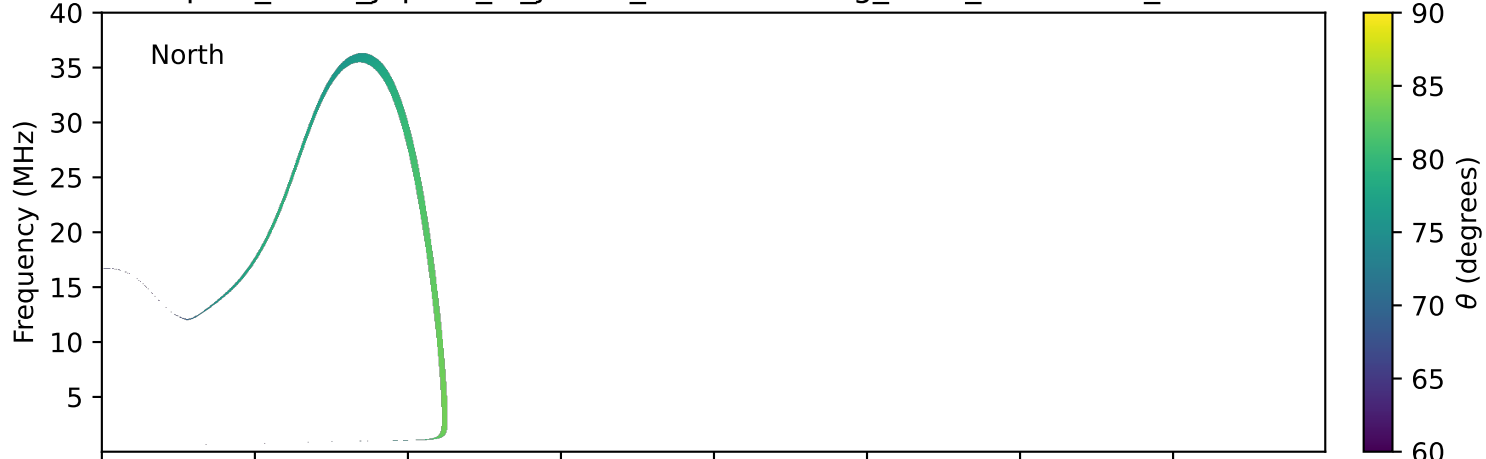
expres_earth_jupiter_io_jrm33_lossc-wid1deg_3kev_19910704_v11.cdf
