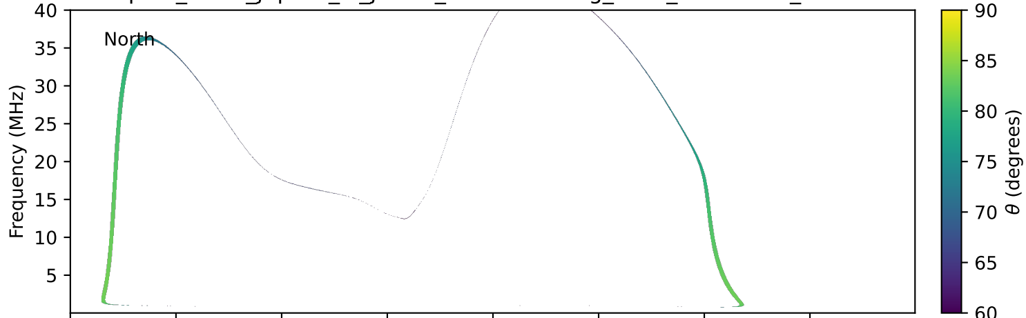
expres_earth_jupiter_io_jrm09_lossc-wid1deg_3kev_19910721_v11.cdf
