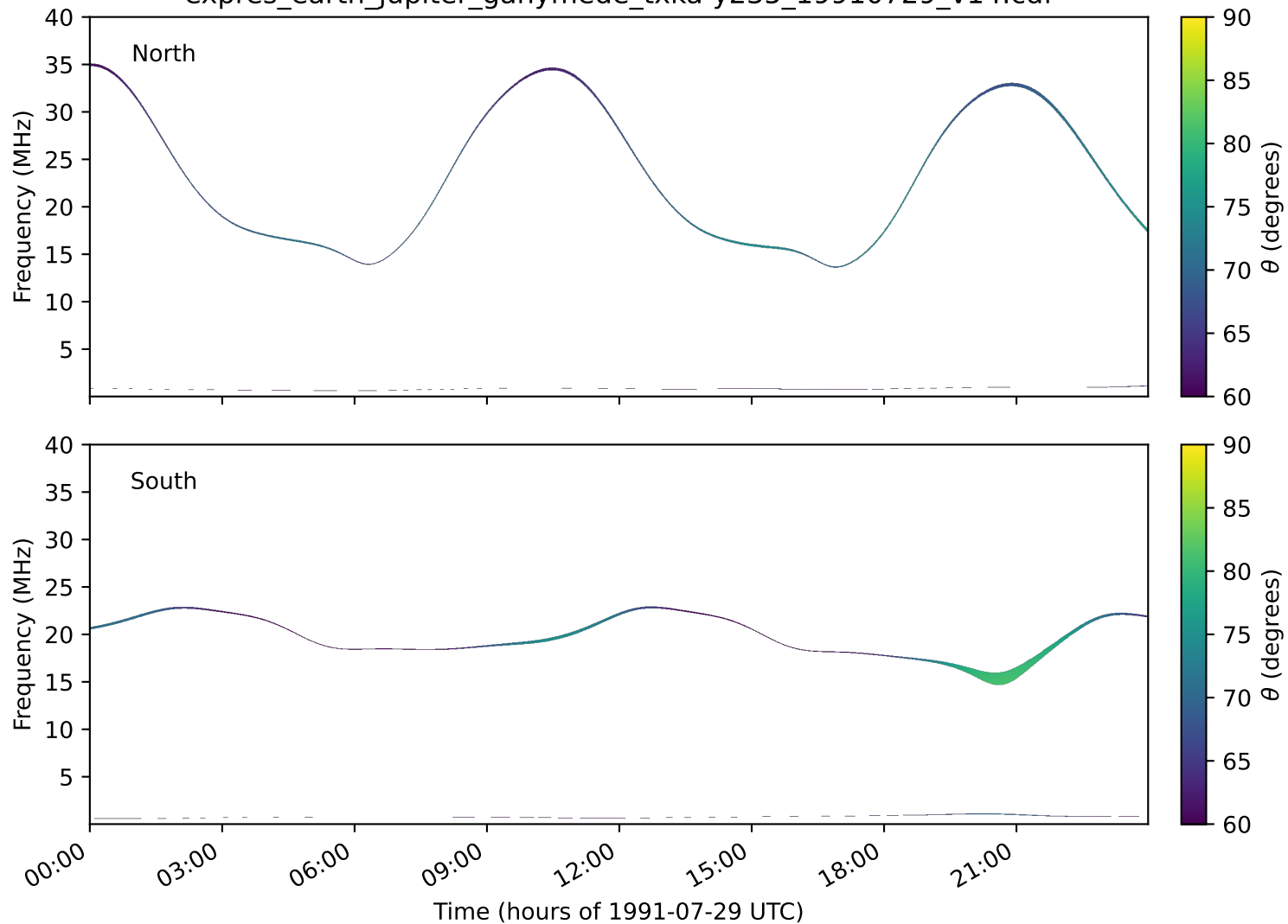
expres_earth_jupiter_ganymede_txka-y235_19910729_v14.cdf
