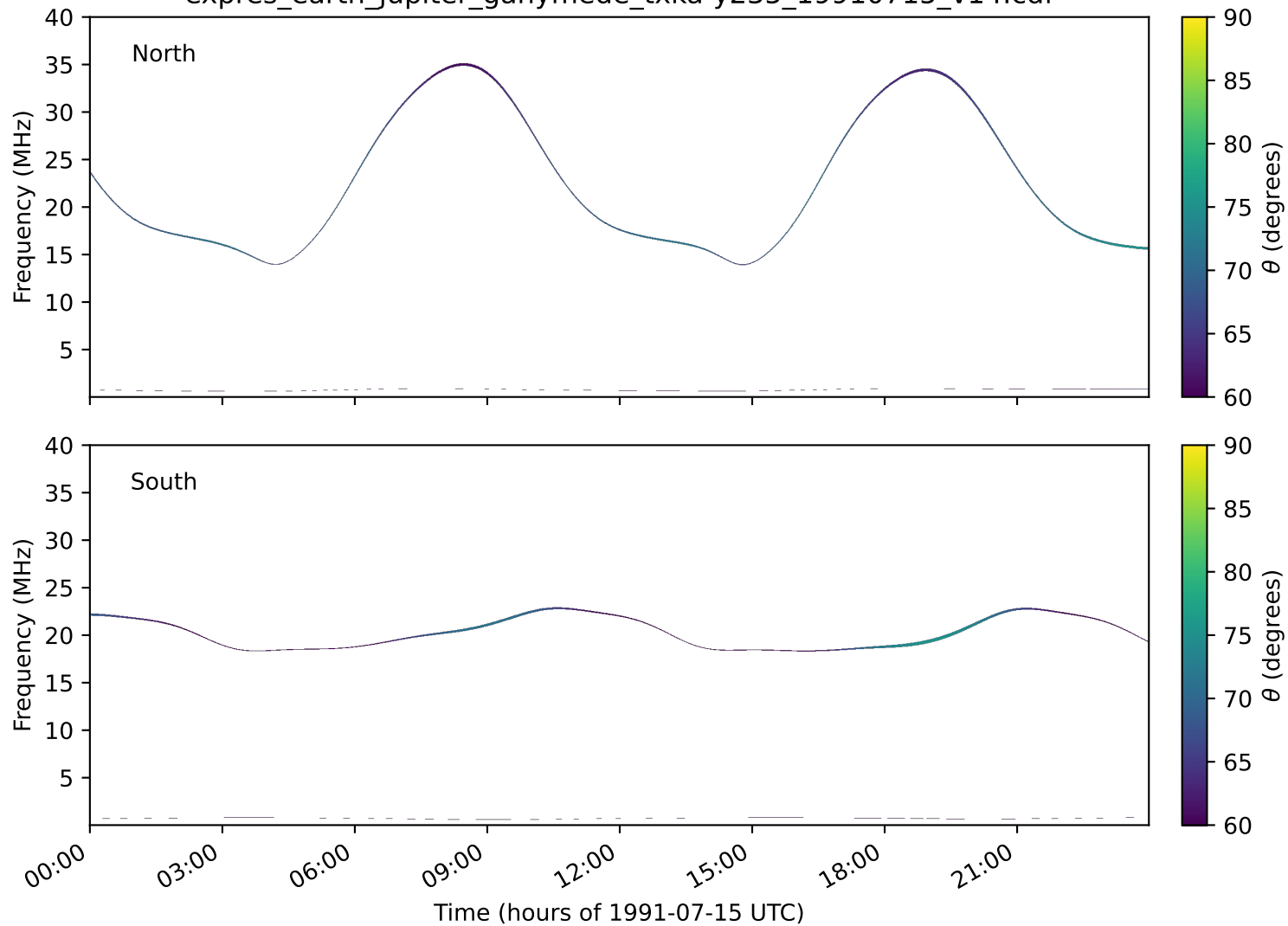
expres_earth_jupiter_ganymede_txka-y235_19910715_v14.cdf
