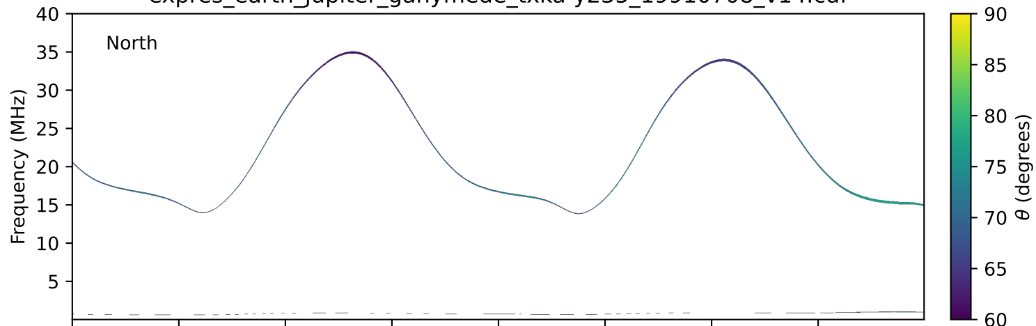
expres_earth_jupiter_ganymede_txka-y235_19910708_v14.cdf
