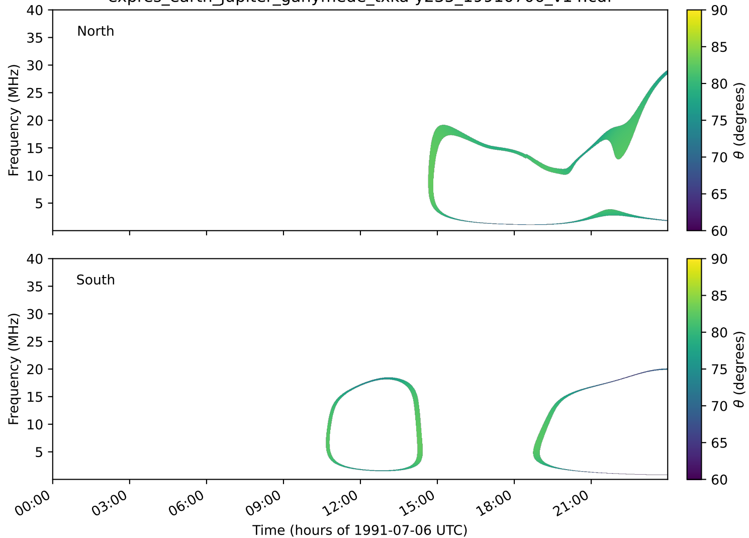
expres_earth_jupiter_ganymede_txka-y235_19910706_v14.cdf
