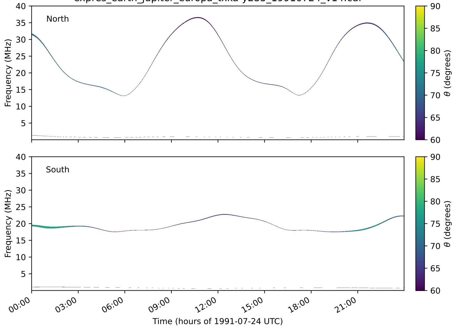
expres_earth_jupiter_europa_txka-y235_19910724_v14.cdf
