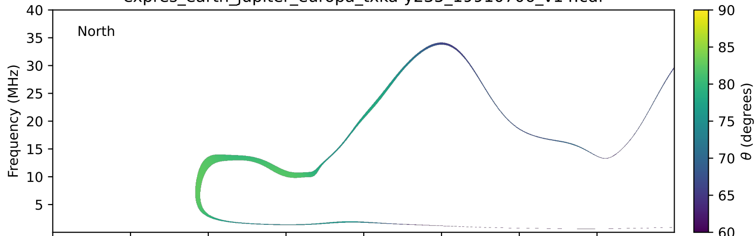
expres_earth_jupiter_europa_txka-y235_19910706_v14.cdf
