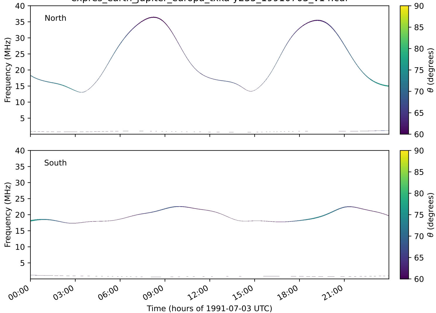
expres_earth_jupiter_europa_txka-y235_19910703_v14.cdf
