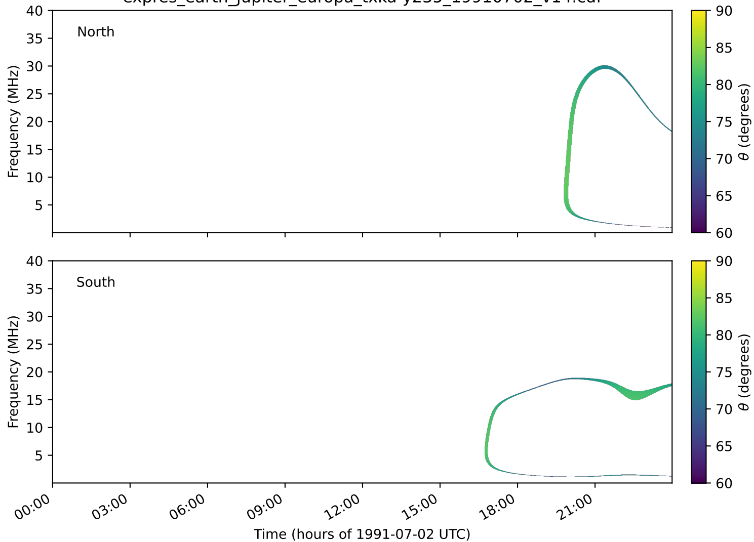
expres_earth_jupiter_europa_txka-y235_19910702_v14.cdf
