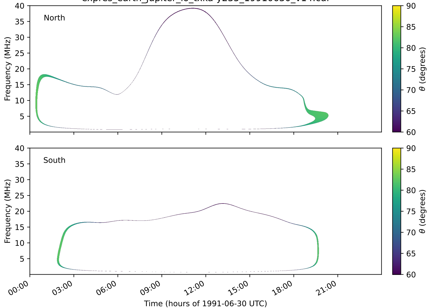
expres_earth_jupiter_io_txka-y235_19910630_v14.cdf
