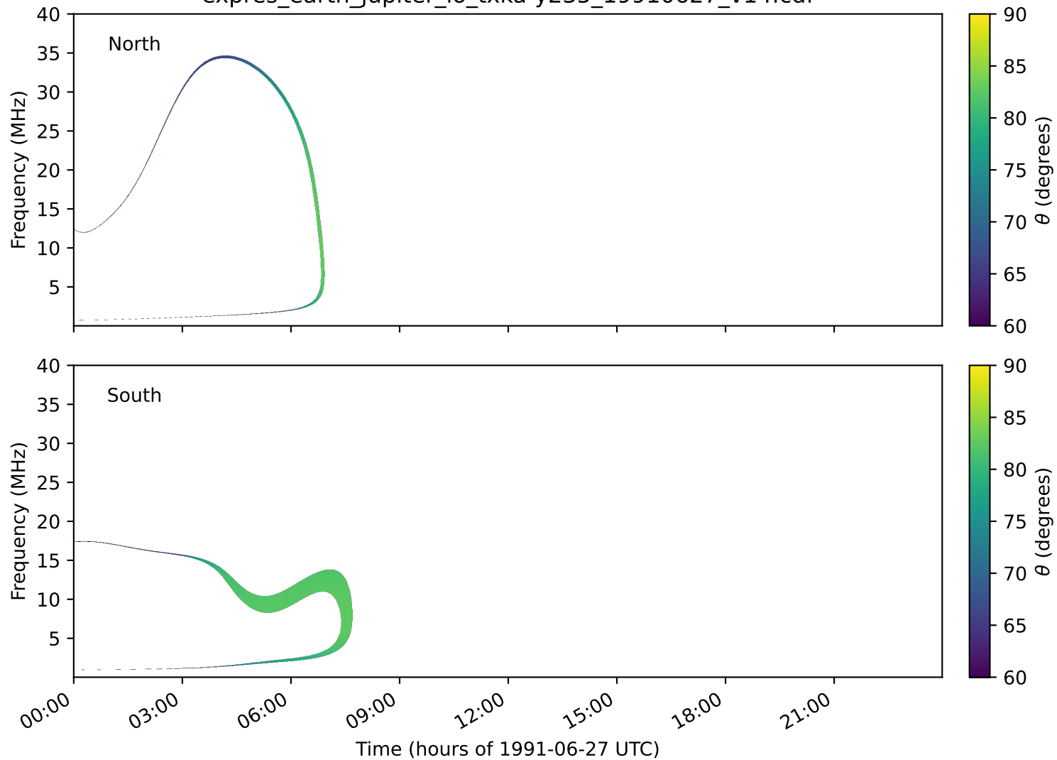
expres_earth_jupiter_io_txka-y235_19910627_v14.cdf
