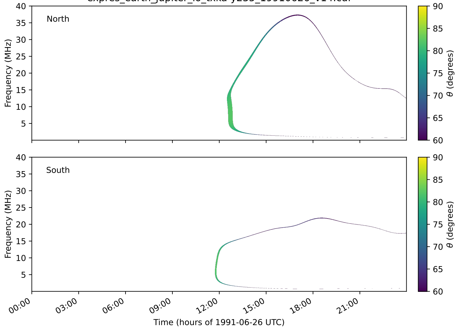
expres_earth_jupiter_io_txka-y235_19910626_v14.cdf
