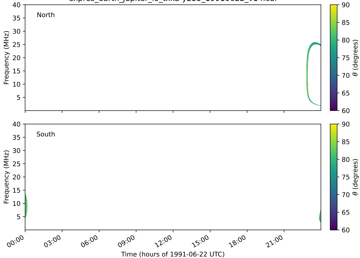
expres_earth_jupiter_io_txka-y235_19910622_v14.cdf
