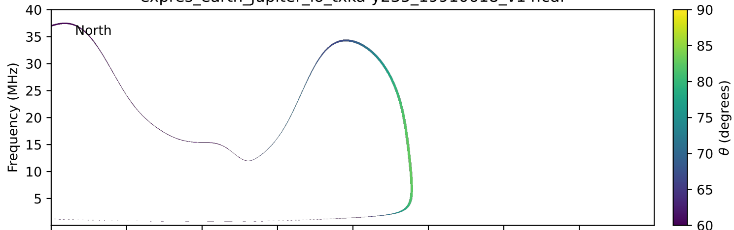
expres_earth_jupiter_io_txka-y235_19910618_v14.cdf
