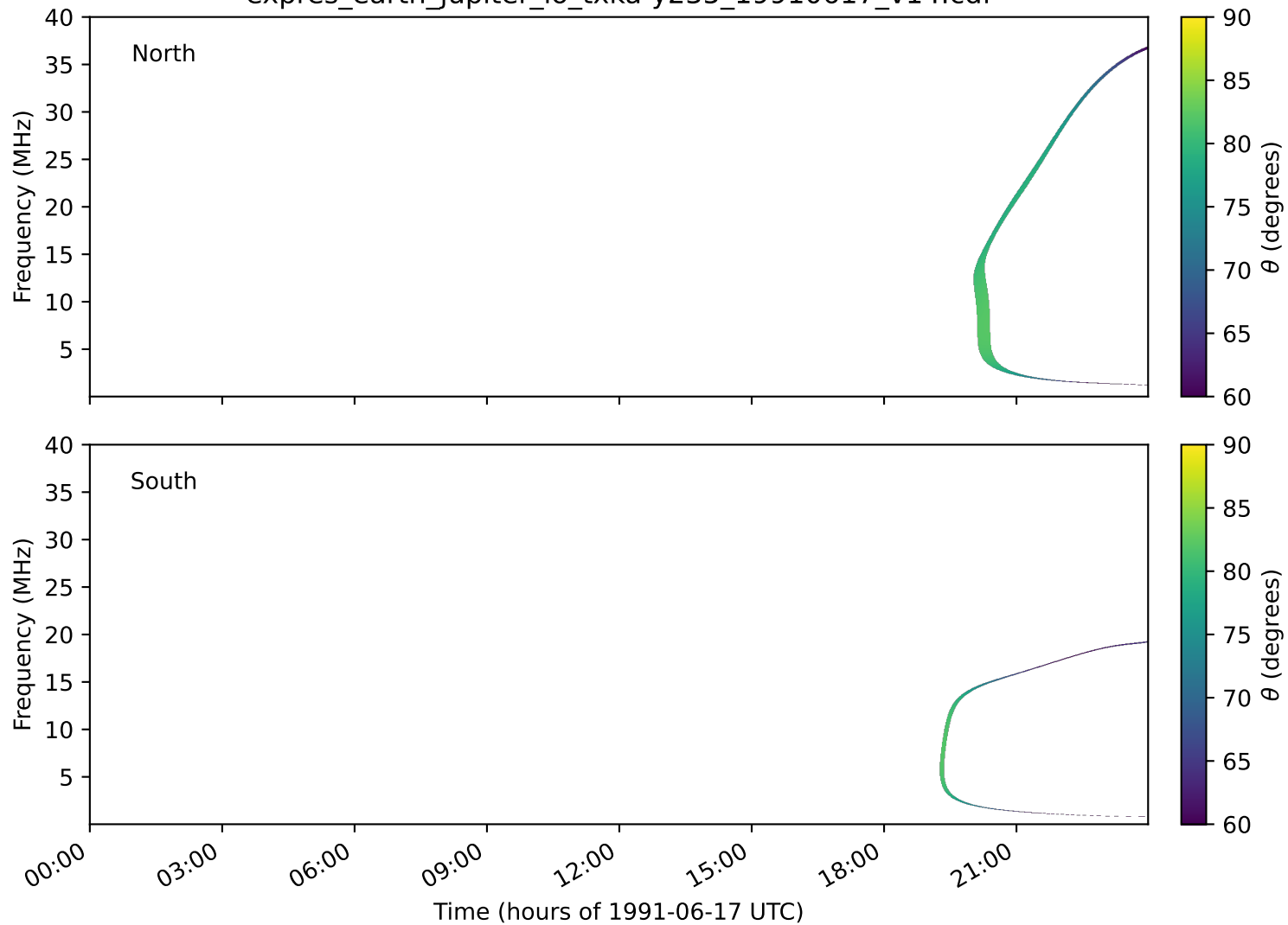
expres_earth_jupiter_io_txka-y235_19910617_v14.cdf
