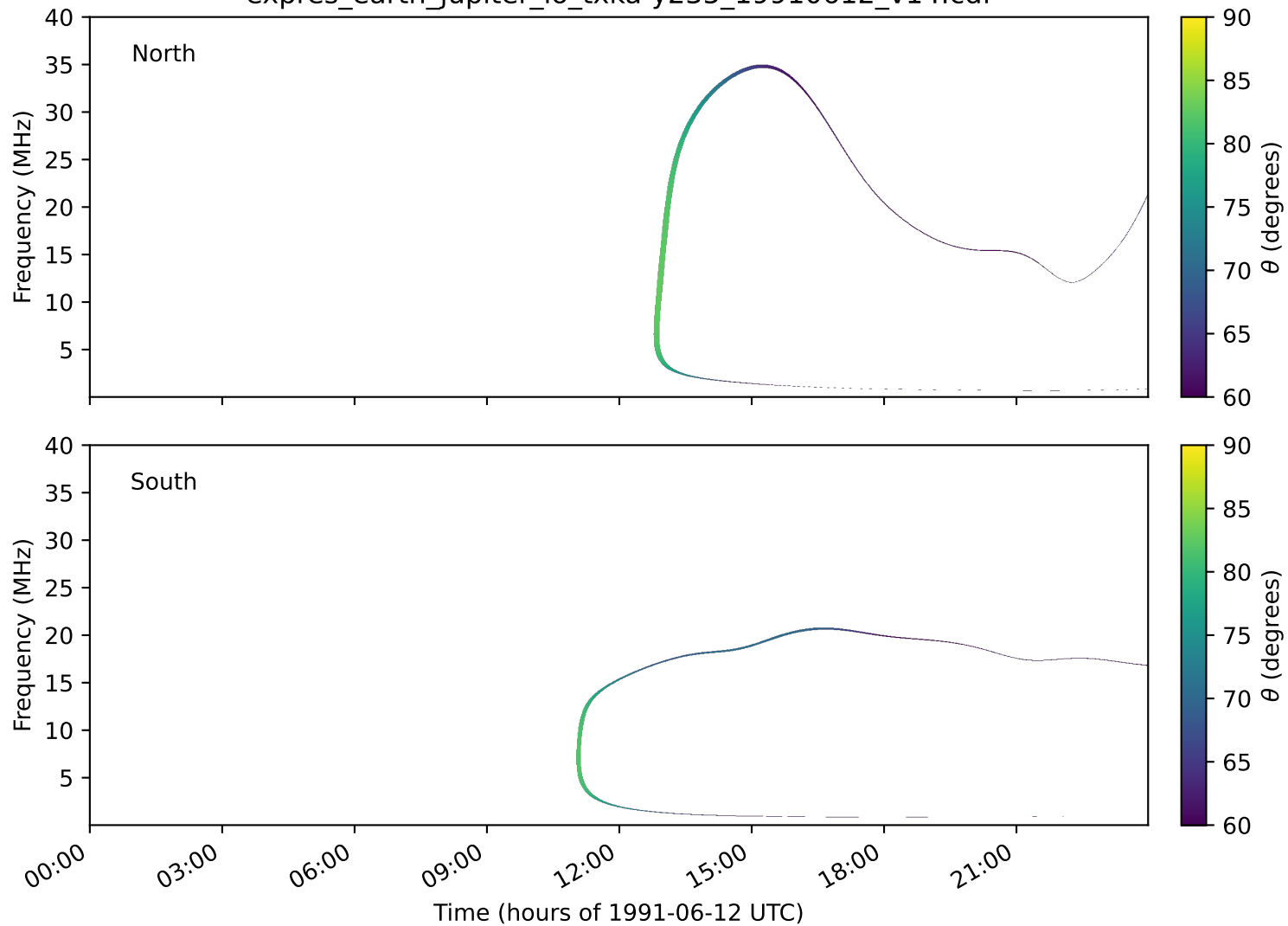
expres_earth_jupiter_io_txka-y235_19910612_v14.cdf
