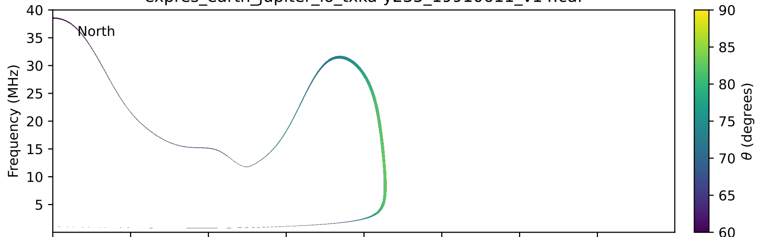
expres_earth_jupiter_io_txka-y235_19910611_v14.cdf
