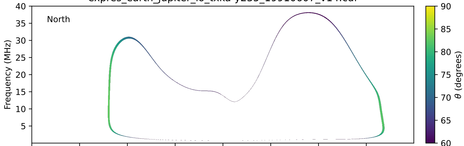
expres_earth_jupiter_io_txka-y235_19910607_v14.cdf
