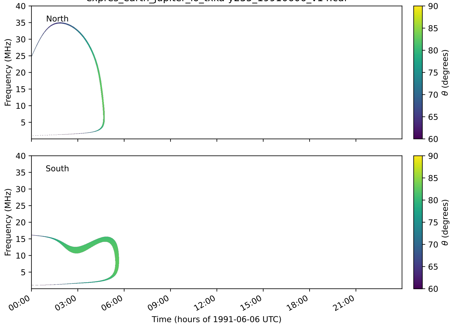
expres_earth_jupiter_io_txka-y235_19910606_v14.cdf
