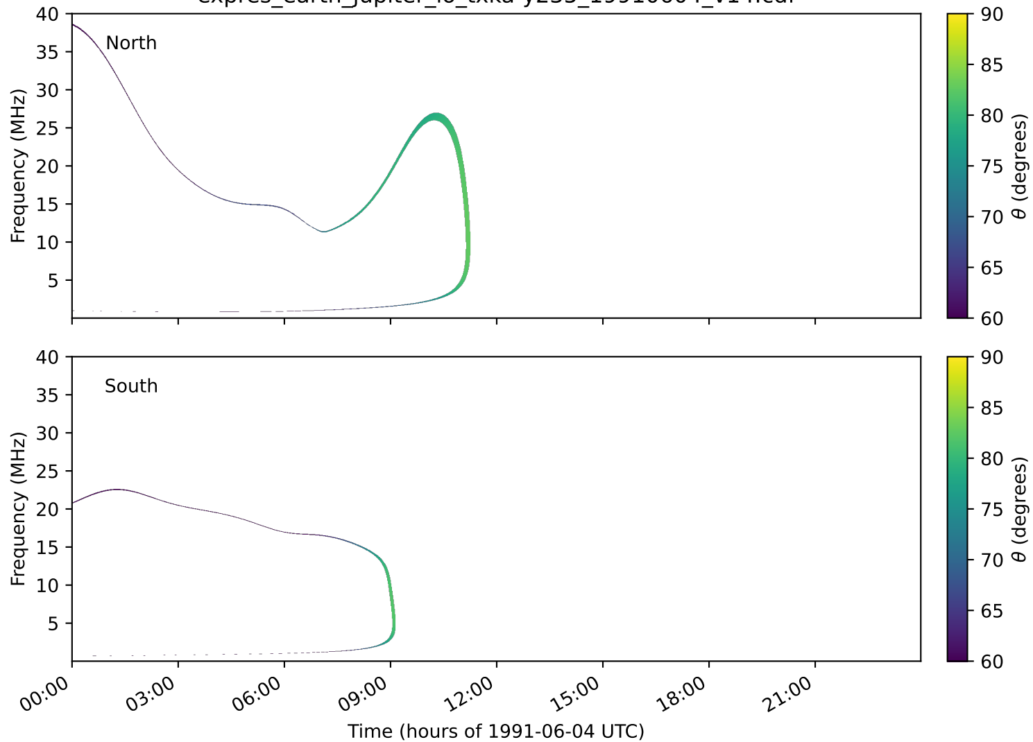
expres_earth_jupiter_io_txka-y235_19910604_v14.cdf
