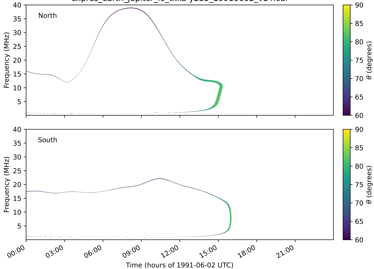
expres_earth_jupiter_io_txka-y235_19910602_v14.cdf
