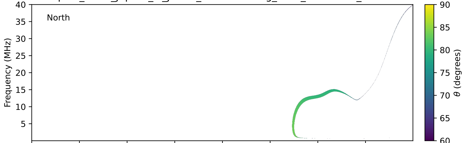
expres_earth_jupiter_io_jrm33_lossc-wid1deg_3kev_19910624_v11.cdf
