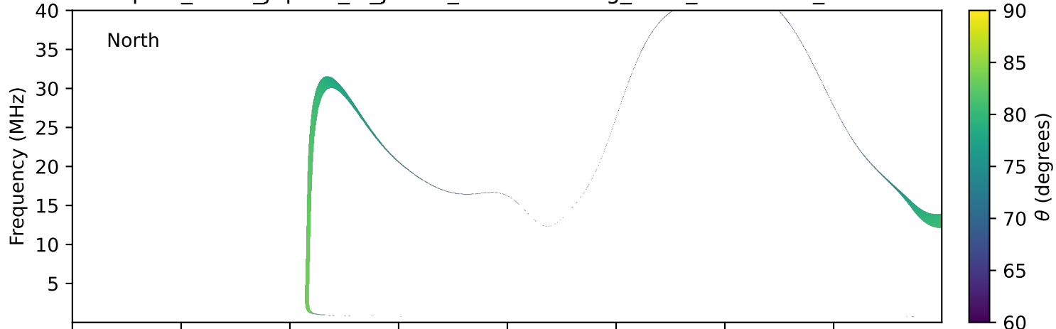
expres_earth_jupiter_io_jrm33_lossc-wid1deg_3kev_19910614_v11.cdf
