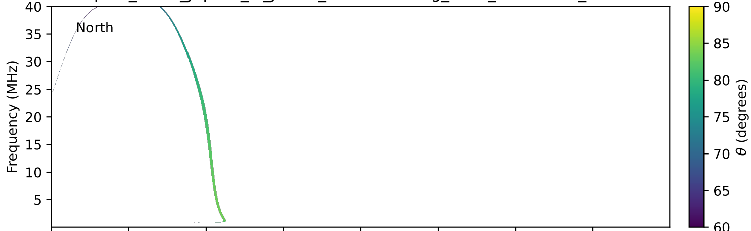
expres_earth_jupiter_io_jrm33_lossc-wid1deg_3kev_19910613_v11.cdf
