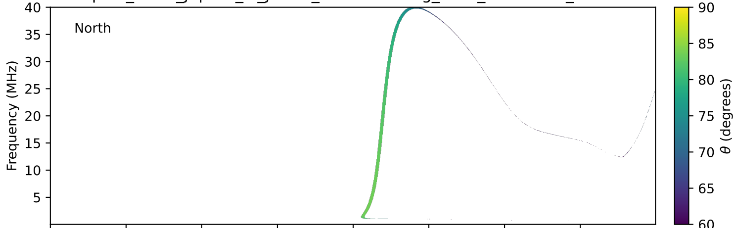
expres_earth_jupiter_io_jrm09_lossc-wid1deg_3kev_19910612_v11.cdf
