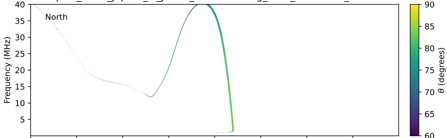
expres_earth_jupiter_io_jrm09_lossc-wid1deg_3kev_19910611_v11.cdf
