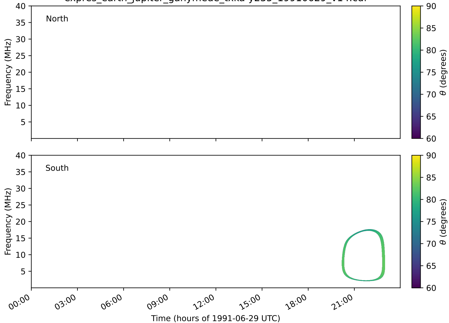
expres_earth_jupiter_ganymede_txka-y235_19910629_v14.cdf
