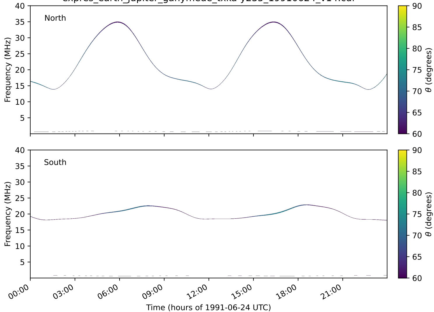
expres_earth_jupiter_ganymede_txka-y235_19910624_v14.cdf
