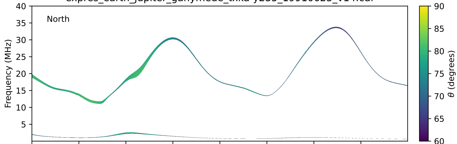
expres_earth_jupiter_ganymede_txka-y235_19910623_v14.cdf
