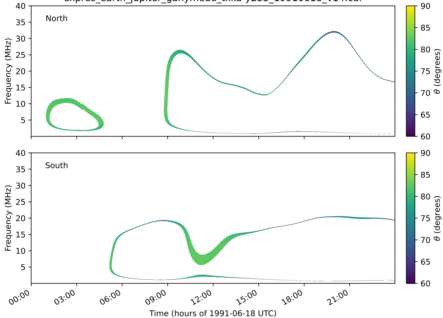
expres_earth_jupiter_ganymede_txka-y235_19910618_v14.cdf
